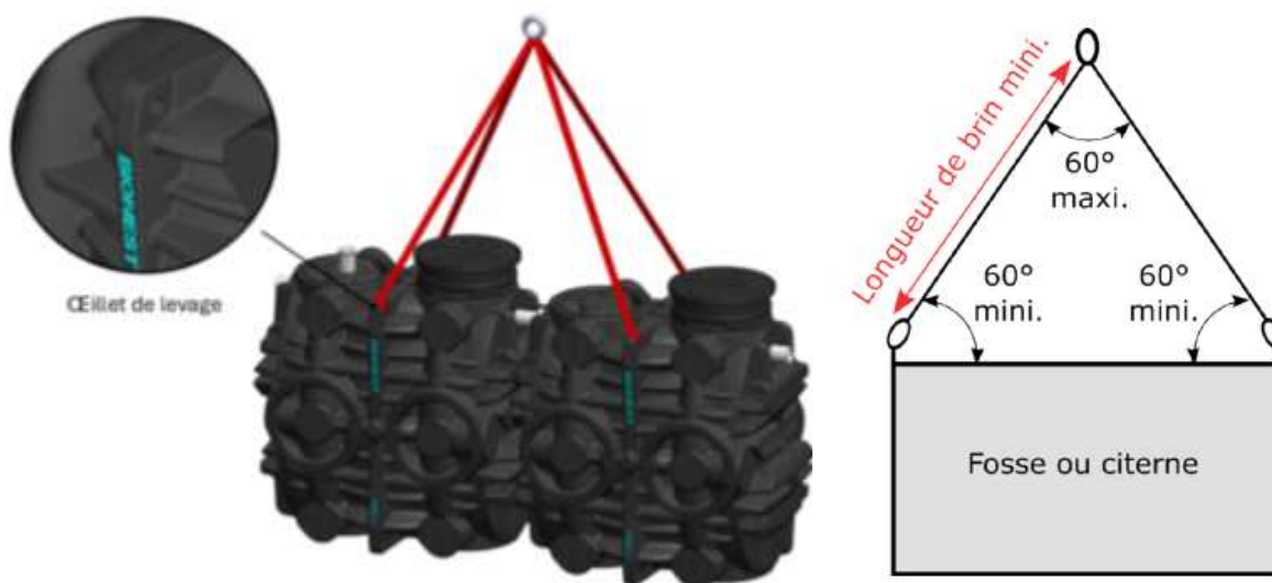
Figure 22: Manutention des cuves PE
