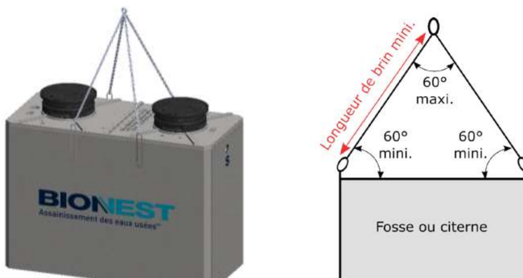
Figure 20: Manutention des cuves béton
