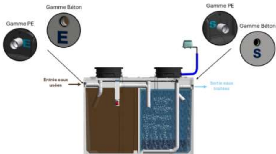
Figure 34: Indications de raccordement hydraulique
